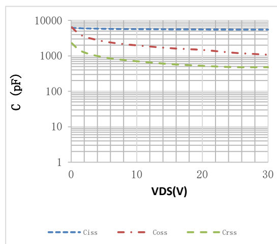
Fig.2 Capacitance Characteristics
